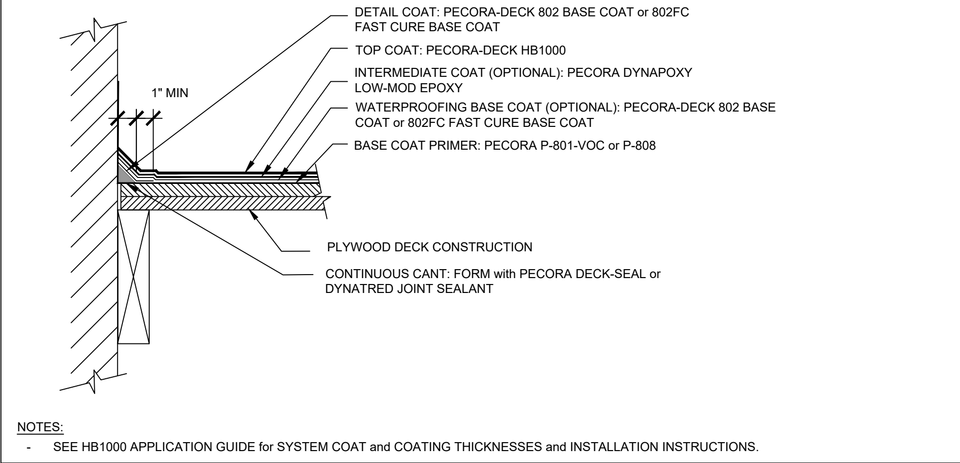
122: PLYWOOD DECK-TO-WALL STATIC JOINT
