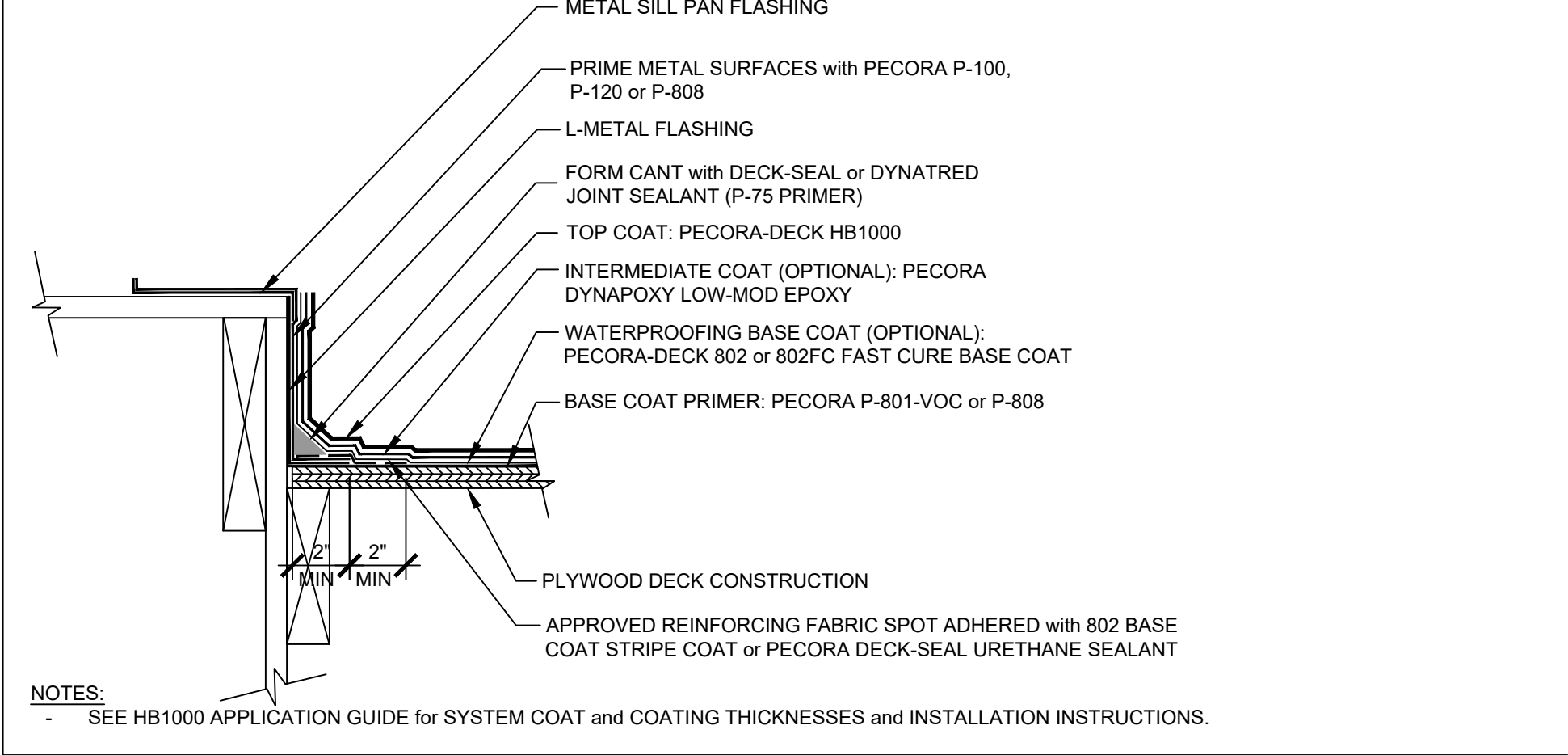
122A: PLYWOOD DECK FLASHING TIE-IN
